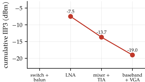
linearity: set by the last stage
