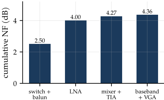
noise: settled by the LNA
