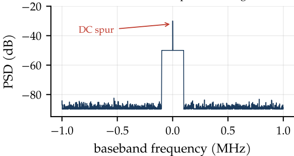
tuned dead centre: spur on the signal
