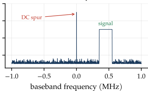
LO offset 450 kHz: spur outside it
