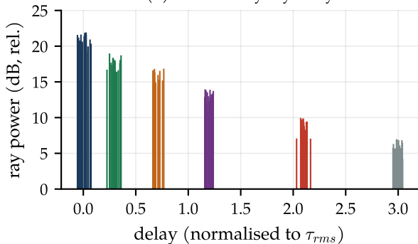
(b) the same rays by delay
