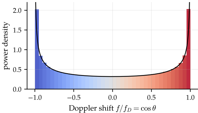
(b) uniform angles pile up at \pm f_D : the 'bathtub'
