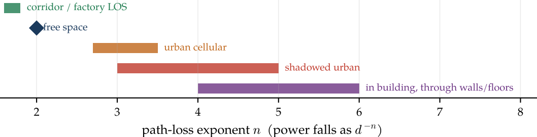
Measured path-loss exponents by environment (typical ranges)
