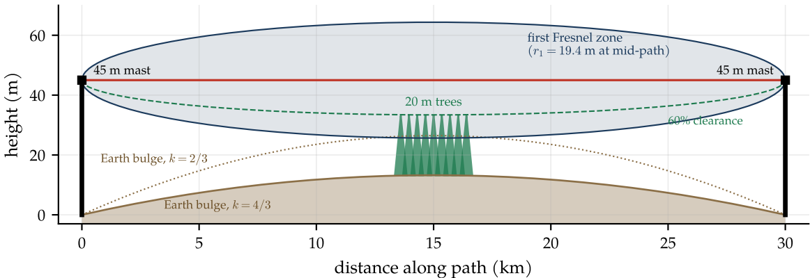
A 30 km, 6 GHz hop: the 'football' must clear trees and the curved Earth (vertical scale exaggerated)
