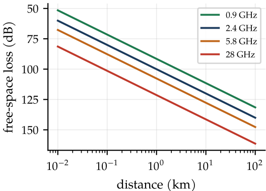
20 dB per decade, isotropic antennas
