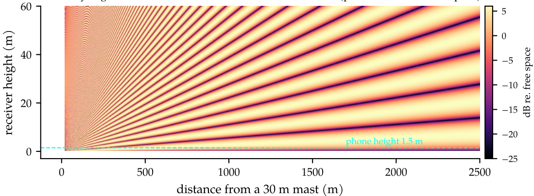
Direct ray + ground reflection at 900 MHz: interference lobes (power relative to free space)
