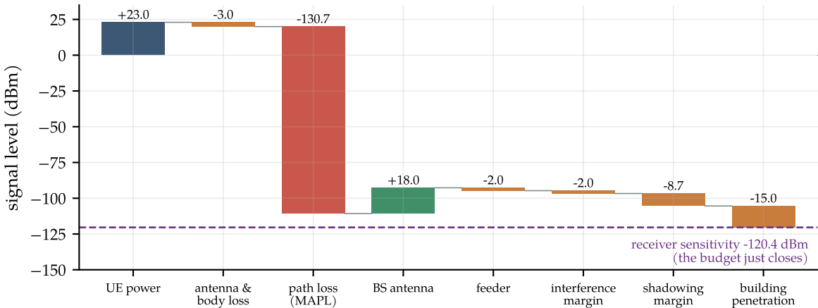
The LTE uplink budget of Table 11.1 as a waterfall
