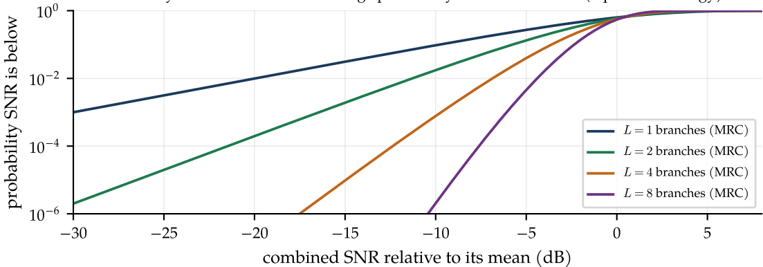
Diversity hardens the channel: outage probability of L -branch MRC (equal total energy)
