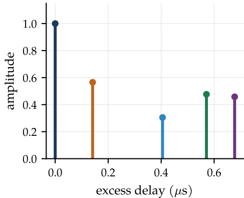
(b) what the phone receives: an impulse response
