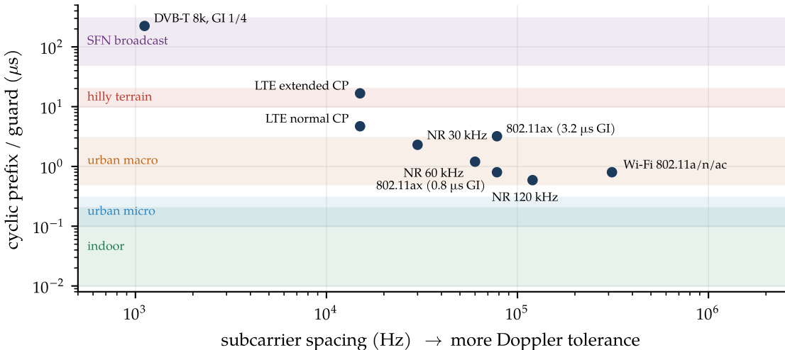
OFDM numerologies versus the delay spreads they must cover
