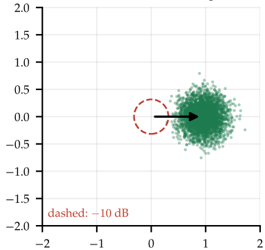
(c) Rician K = 10 : strong LOS
