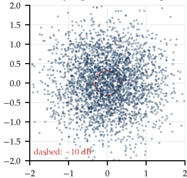
(b) Rayleigh: no dominant path
