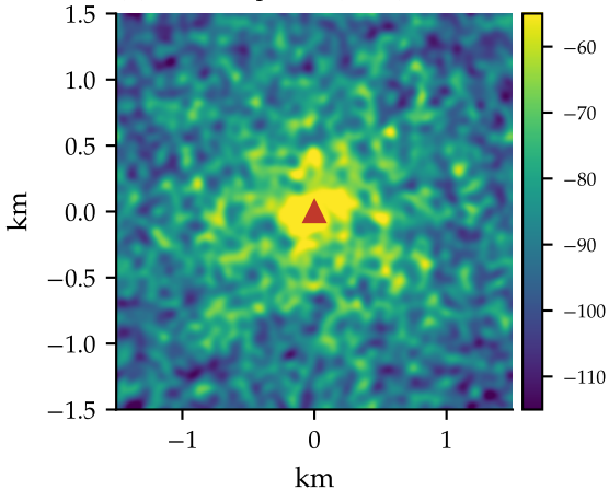
(a) received power (dBm), \sigma = 8 dB
