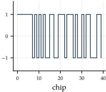
(a) transmitted PN chips
