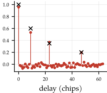
(c) correlate the echo: h(\tau) appears
