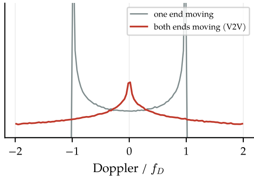
(b) vehicle-to-vehicle Doppler spectrum
