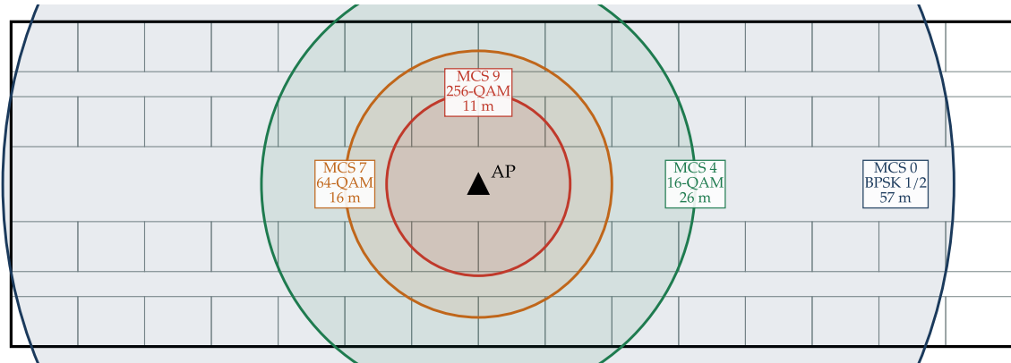
Approximate 802.11ac range rings through interior walls (3GPP InH NLOS model, 5.5 GHz)
