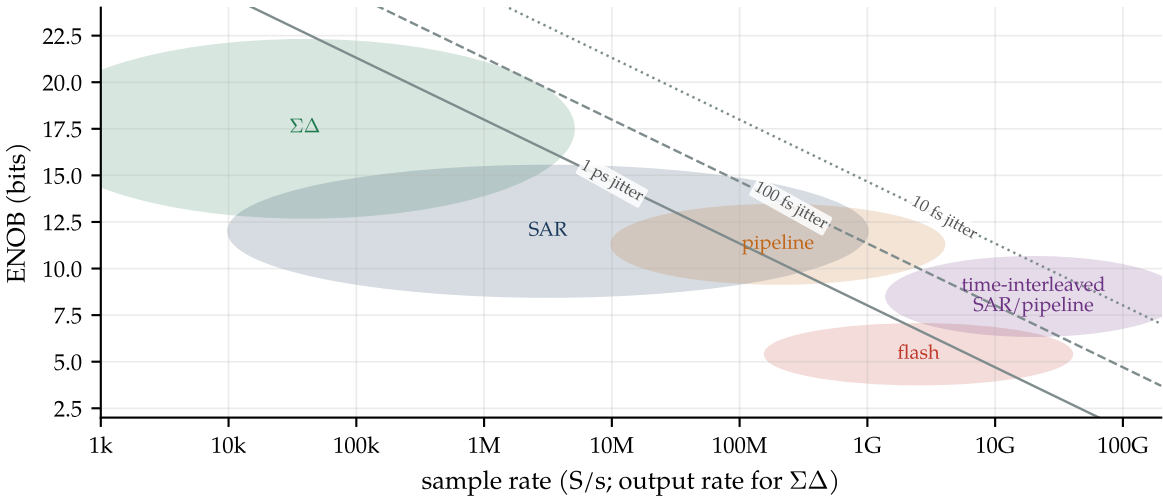
The converter landscape (approximate regions) and the jitter wall at Nyquist input
