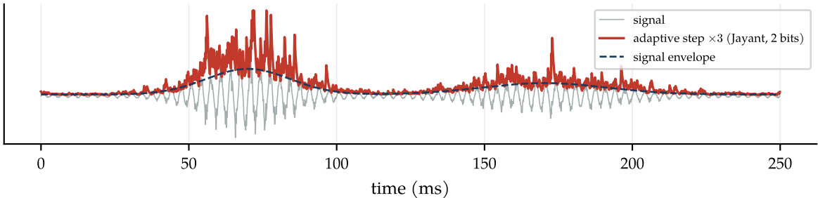
Backward adaptation: the step follows the loudness, with no side information
