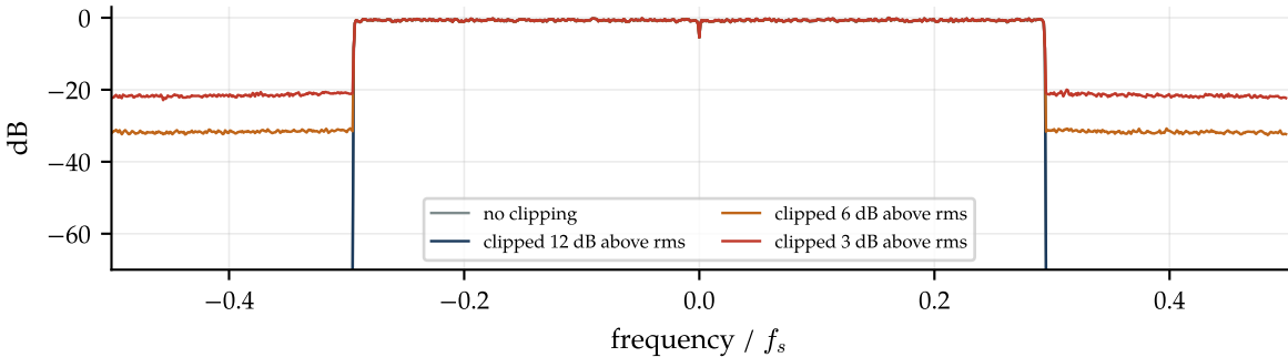
Clipping an OFDM signal: the spectrum splatters into the neighbours
