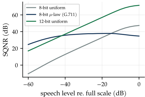
SQNR with Laplacian (speech-like) input
