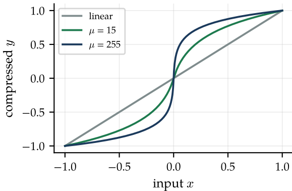
\mu -law compression characteristic
