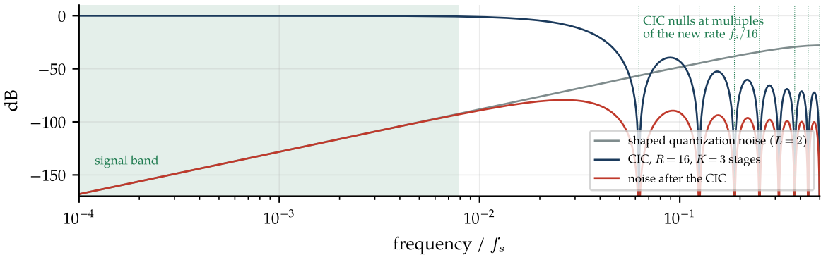
The first decimation stage: a CIC kills the noise exactly where it would alias
