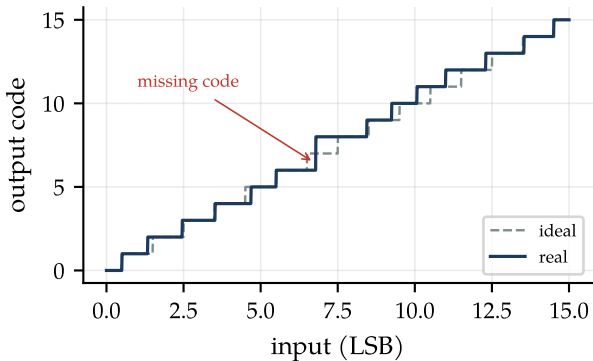
A 4-bit staircase with errors
