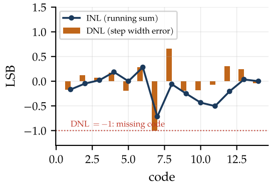
DNL and INL
