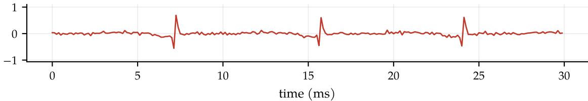
order-10 prediction error: variance 10.5 dB smaller, crest factor 10.3
