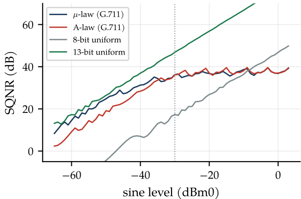
Sine-wave SQNR of real G.711 codecs
