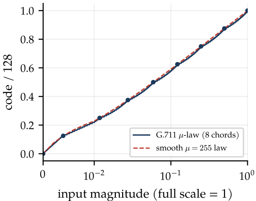
Chords end at x_k = (2^k - 1)/255
