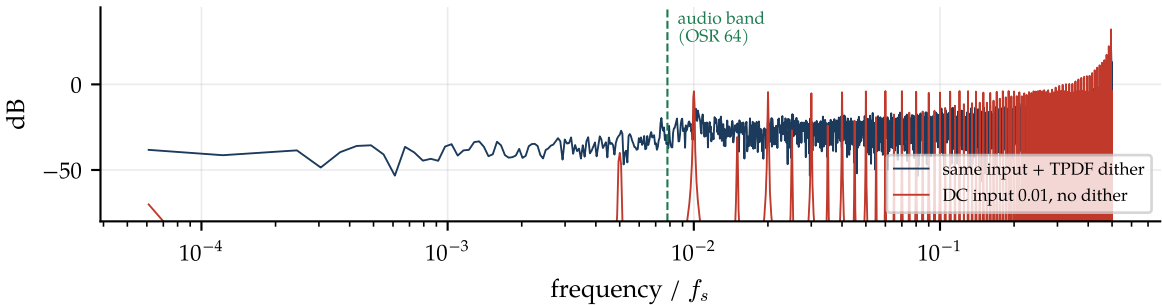
Idle tones: a first-order loop with a constant input sings a periodic pattern
