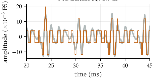
8-bit uniform: SQNR 7 dB
