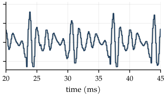
8-bit \mu -law: SQNR 34 dB
