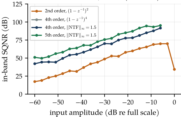
1-bit modulators, OSR 64 (simulated)
