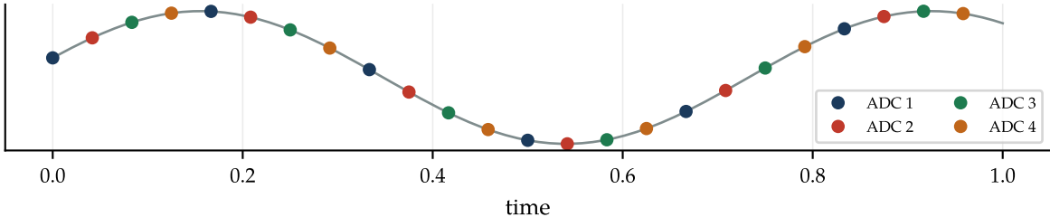
Time interleaving: four slow converters take turns, each sampling every fourth instant
