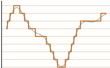
(b) quantization: amplitude made discrete (always loses a little)
