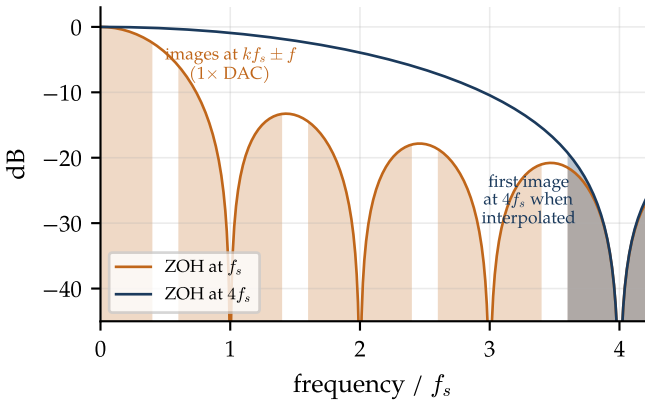
Images and sinc envelope (signal band 0-- 0.4f_s )
