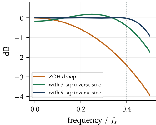
Droop and its correction
