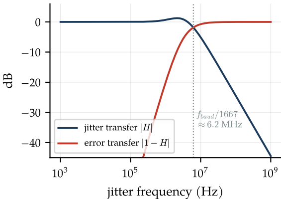
(a) CDR loop, 10.3125 GBd
