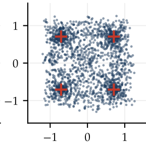
clock offset 250 ppm
