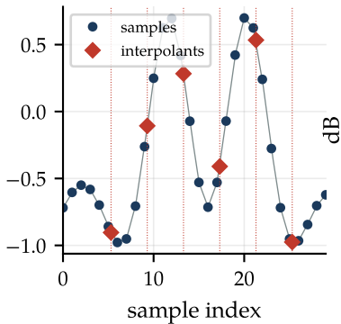
(a) strobes at m_k + \mu_k
