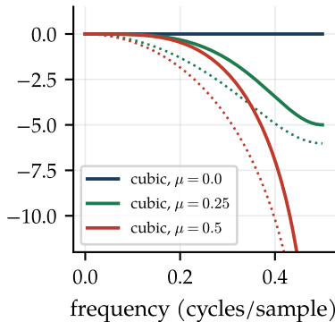
(b) magnitude (dotted: linear)
