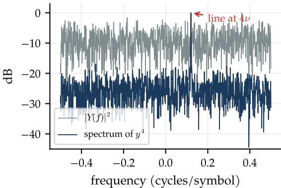
(a) QPSK, \nu = 0.03 , E_s/N_0 = 10 dB
