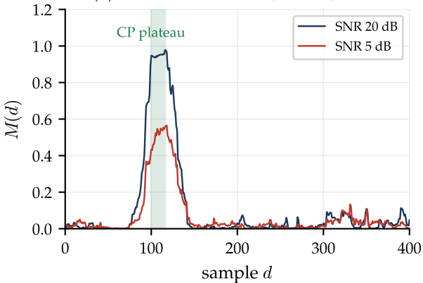
(a) Schmidl--Cox metric, N = 64 , CP 16
