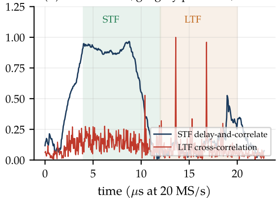
(b) IEEE 802.11a/g legacy preamble, 10 dB
