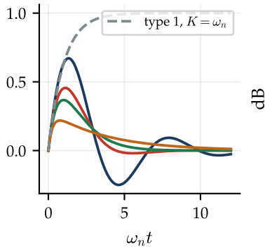
(b) frequency step \Delta\omega : \theta_e \omega_n / \Delta\omega
