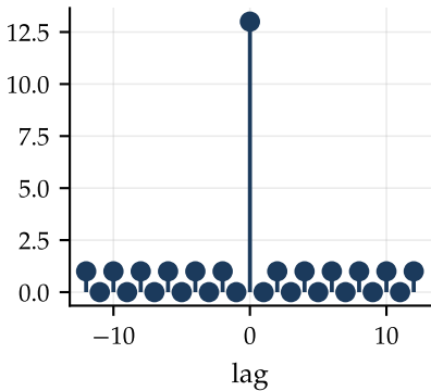
(a) Barker-13, aperiodic
