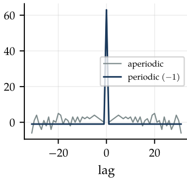
(b) m-sequence, N = 63
