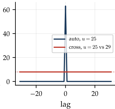
(c) Zadoff-Chu, N = 63 , periodic
