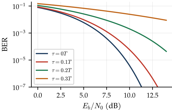
(a) QPSK, RC \beta = 0.35 , static offset
