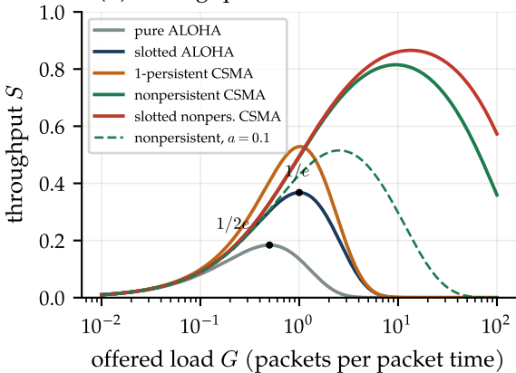
(a) throughput, a = 0.01 unless stated
