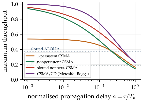
(b) capacity versus a
