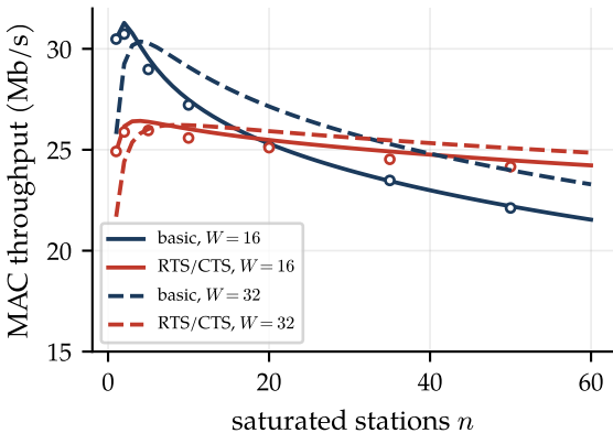
(a) 802.11a, 54 Mb/s, 1500-byte frames
