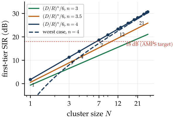
(a) co-channel SIR at the cell edge
