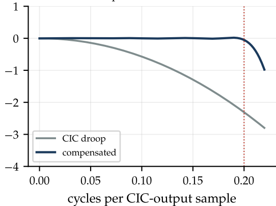
passband detail
