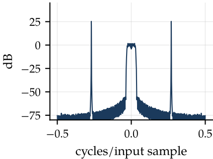
input: band at \pm 0.03 , tone at 0.27
