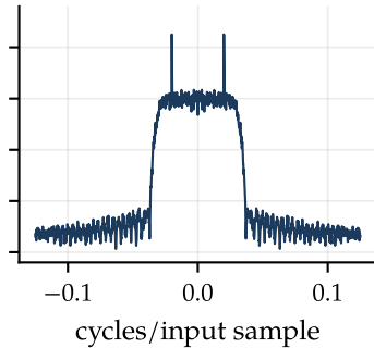
naive downsample by 4: tone aliases in-band
