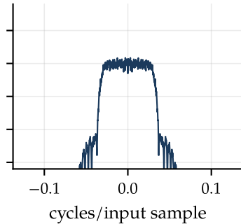
filter first, then downsample
