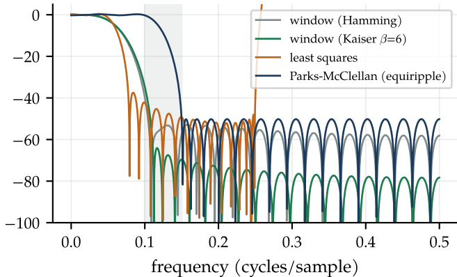
41-tap low-pass designs
