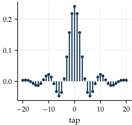
equiripple impulse response
