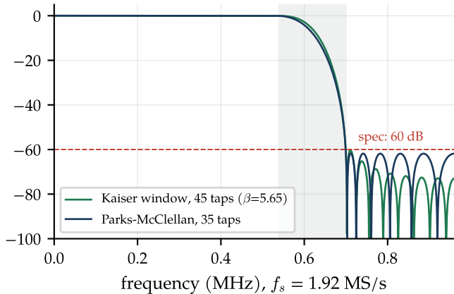
same spec, two designs
