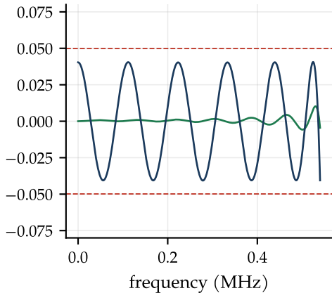
passband detail (spec \pm 0.05 dB)
