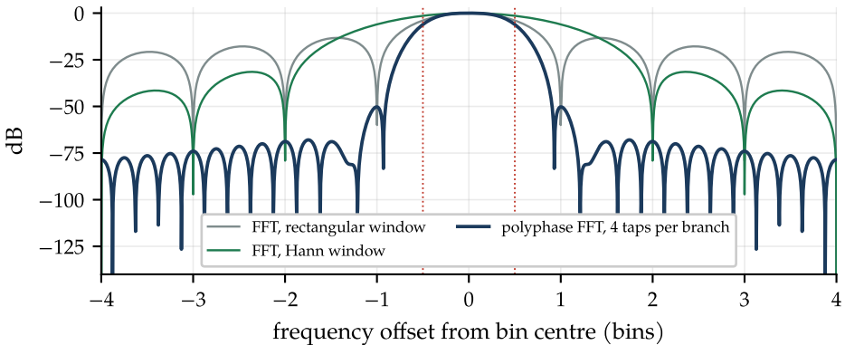
Response of one spectrometer channel
