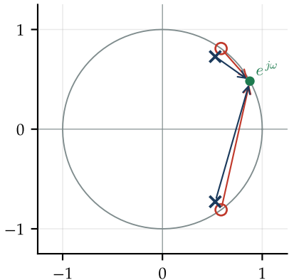
pole-zero geometry ( r = 0.9 )
