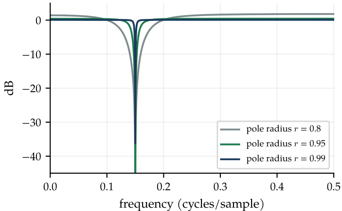
notch at 0.15: bandwidth \approx (1 - r)/\pi cycles/sample
