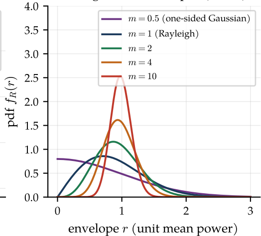
Nakagami- m envelopes ( \Omega = 1 )
