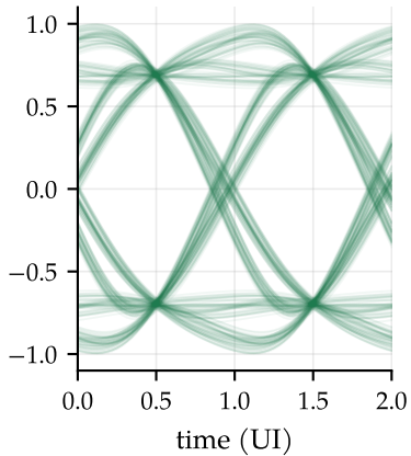
After 9-tap FFE
