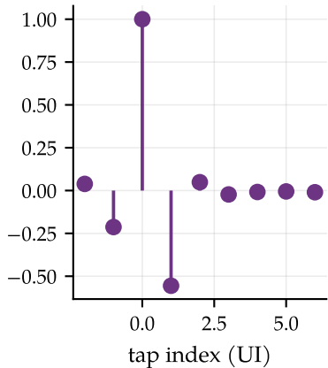
FFE taps (normalized)
